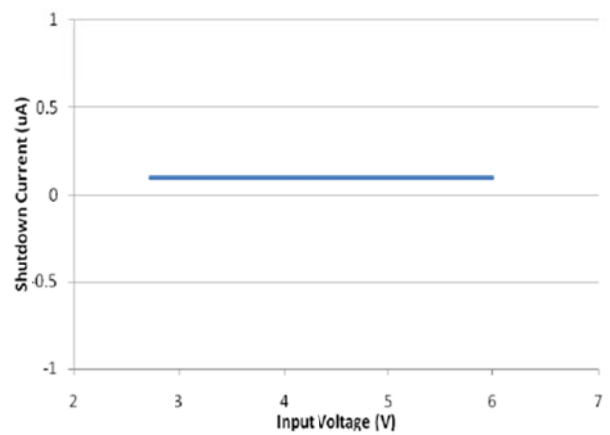
Shutdown Current Vs. Input Voltage V_{IN}=2.7V \sim 6V , V_{EN}=0V , V_{FB}=0.5V
