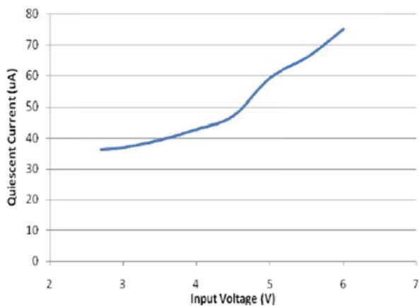
Quiescent Current Vs. Input Voltage V_{IN}=2.7V \sim 6V , V_{EN}=2.5V , V_{FB}=0.8V
